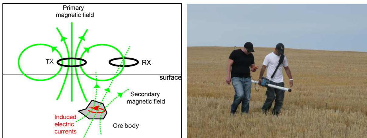
Figure 1: Principle of electromagnetic induction (EM) sounding measurements of the underground conductivity (left, Tx and Rx are the transmitter and receiver coils, respectively); Typical EM measurements with a Geonics EM31MK2 instrument (right; photo by C. Haas @ southern Alberta).
